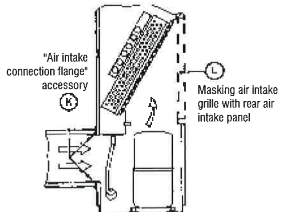
REAR AIR INTAKE (WITH "Air intake connection flange" accessory)
